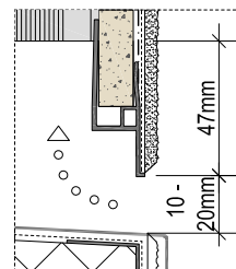
Alternative: ventilation joint with Sto Edge Protection Profile GT
