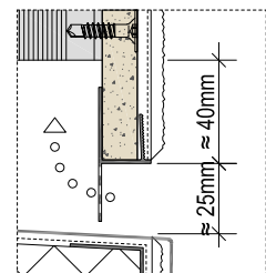
Alternative: ventilation joint with Sto Roof Vent Profile
