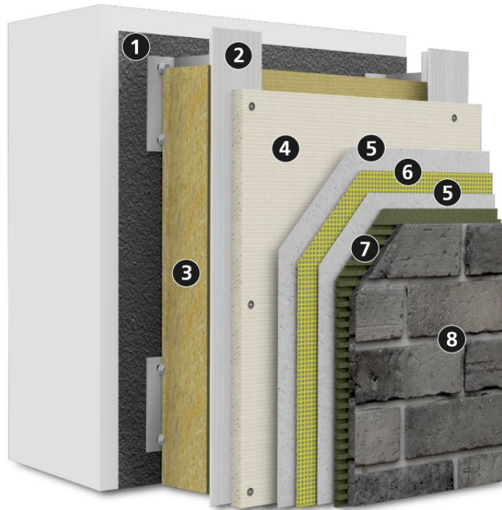
Figure 2 – StoVentec Masonry Vener System
