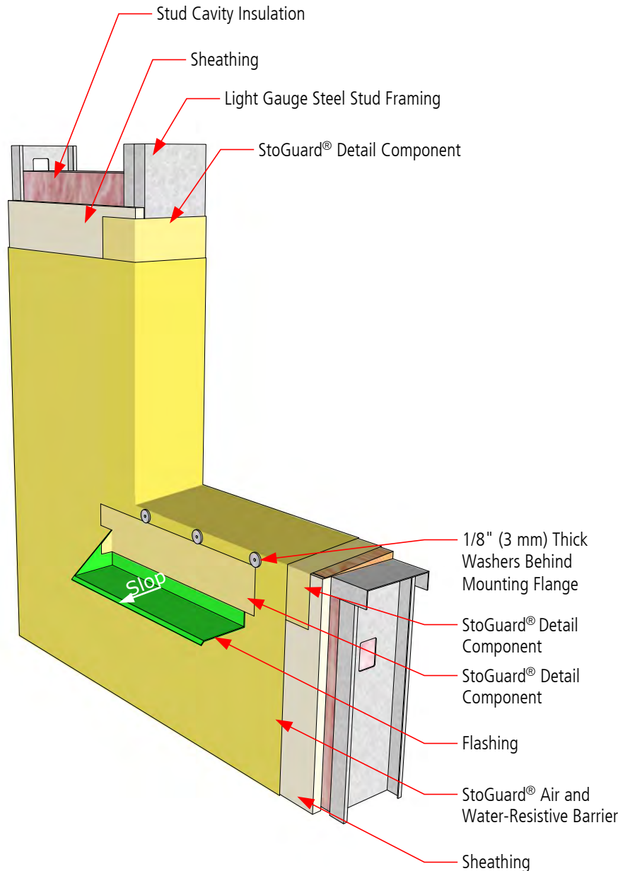
Step 1 - Rough Opening Protection, Sill Flashing
