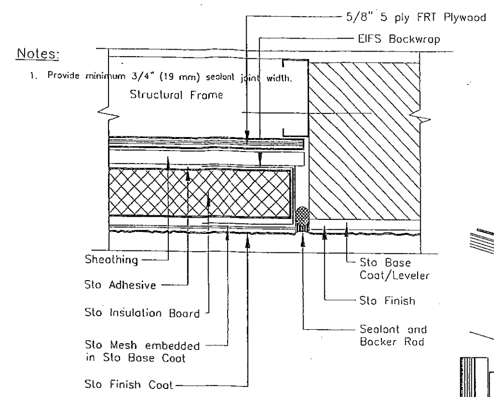
CONSTRUCTION JOINT N.T.S.
