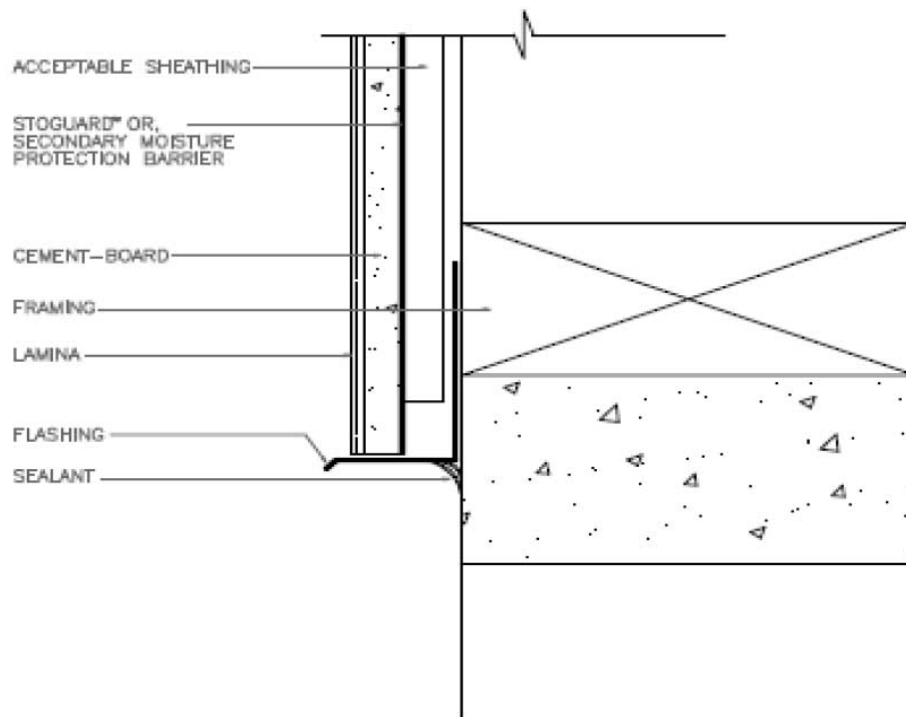
FIGURE 3—TYPICAL TERMINATION AT FOUNDATION
