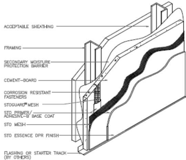
TYPICAL STOQUIK SILVER I CEMENT-BOARD STUCCO SYSTEM
