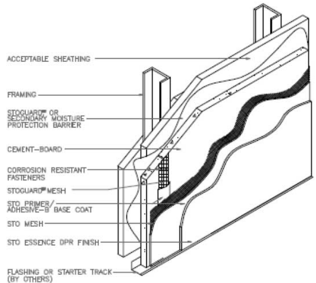
FIGURE 1—STOQUIK™ SILVER I CEMENT-BOARD STUCCO SYSTEM
