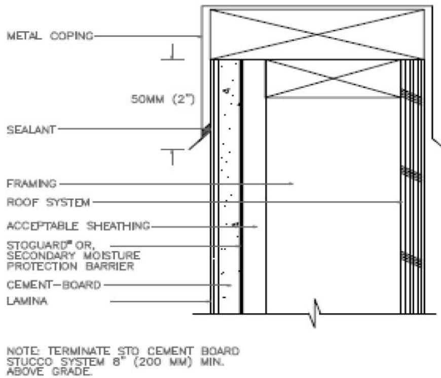
FIGURE 4—TYPICAL METAL COPING DETAIL
